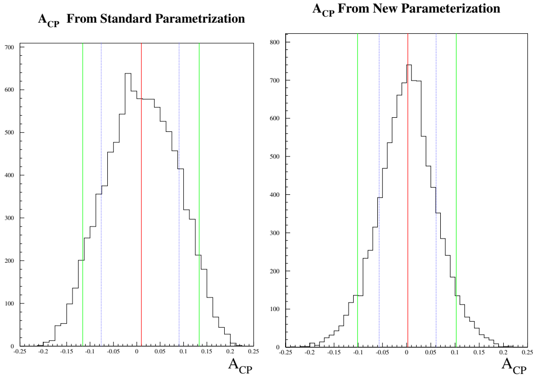
Figure 3.20: The standard parameterization is presented on the left, the new on the right. In both plots, the solid red line in the center is the median value. The dashed blue lines are at \pm 1\sigma and The solid green lines are 90% limit.
