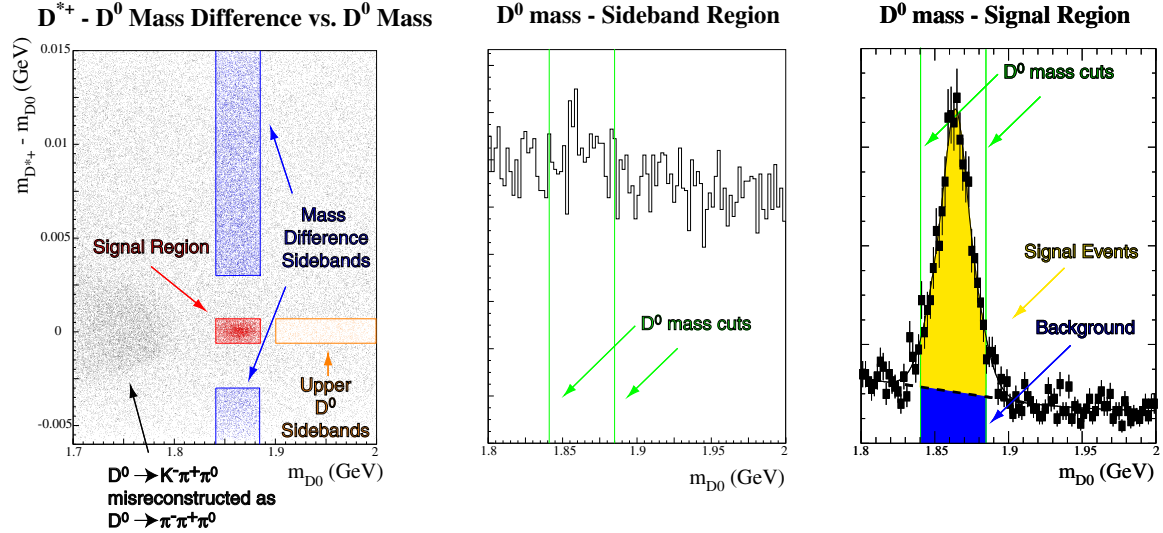
Figure 3.17: We use both the upper and lower mass difference sideband as well as the upper D^0 mass sideband. The middle and right plots show the projections onto the D^0 mass axis for the mass difference sideband and the signal region respectively. Note: The mass difference is centered at the PDG value.
