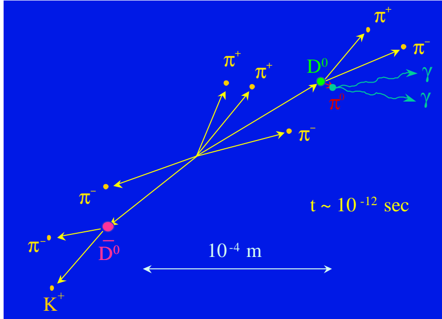
Figure 1.5: After approximately 10^{-12} seconds, weak decays start. In our case, the \bar{D}^0 \rightarrow K^+\pi^- and D^0 \rightarrow \pi^-\pi^+\pi^0 . On the weak time scale, the \pi^0 decays almost immediately (since it decays electromagnetically) into two photons.
