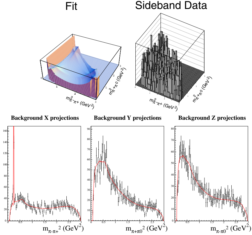
Figure 3.18: The background fit and the sideband data it was fit to. For the projections, the red line is the fit and the black histogram is the data.
