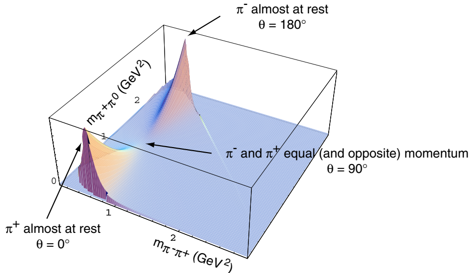
Figure 3.7: |Amplitude|^2 for the vector \pi^-\pi^+ resonance \rho^0 . When the \pi^+ comes out opposite to the \rho^0 direction, it is almost at rest and corresponds to \theta = 0 deg. The \pi^- is almost at rest when \theta = 180 deg. When the pions come out perpendicular to the \rho^0 ( \theta = 90 deg), they have equal momentum. We can see the \cos^2(\theta) dependence mentioned in Figure 3.6.
