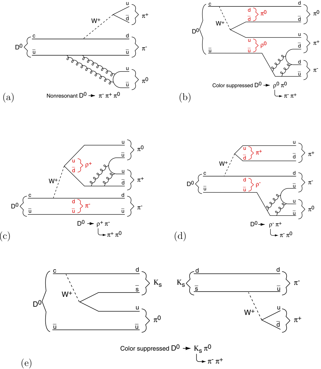
Figure 3.2: Shown are examples of (a) a nonresonant decay, (b) a neutral intermediate state ( \rho^0 ), (c) a positively charged intermediate state ( \rho^+ ), (d) a negatively charged intermediate state ( \rho^- ), and (e) D^0 \rightarrow K_S^0 \pi^0 .
