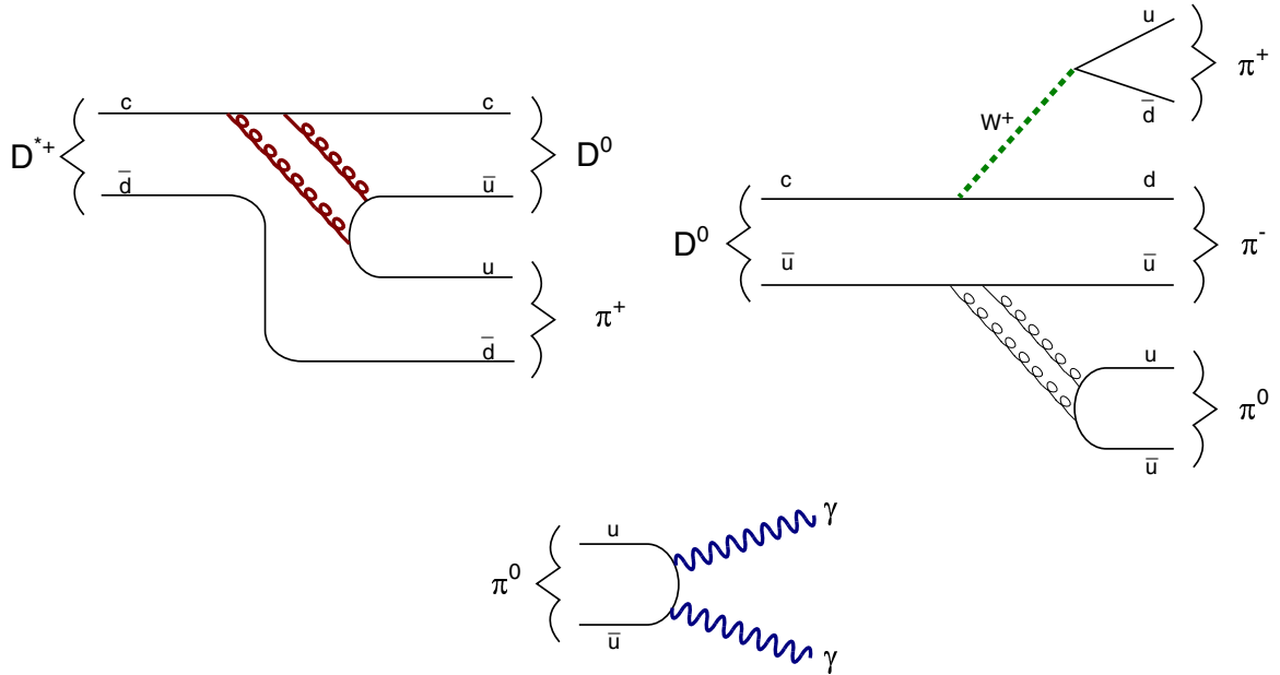
Figure 1.1: Possible Feynman diagrams for the decay chain D^{*+} \rightarrow D^0\pi^+ , D^0 \rightarrow \pi^-\pi^+\pi^0 , \pi^0 \rightarrow \gamma\gamma . The D^{*+} decays strongly , the \pi^0 decays electromagnetically and the D^0 decays weakly .
