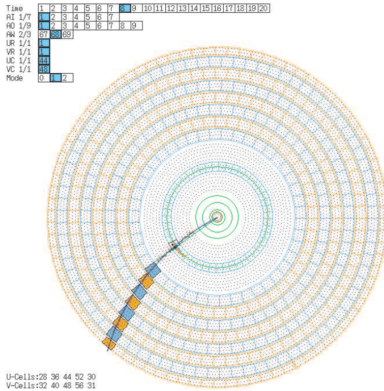
Figure 4.8: The STTR tracks the U superlayers and V superlayers separately. In order for a stereo track to be found, all four blocks (U or V) must be present.
