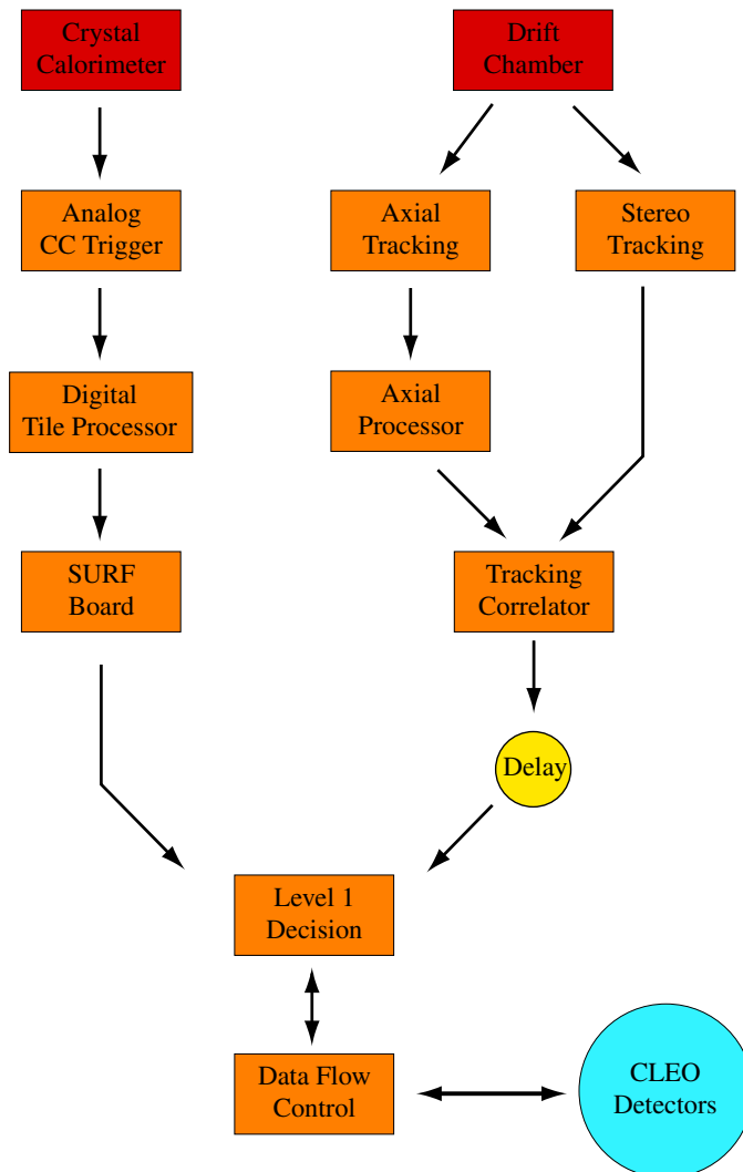
Figure 4.3: An overview of the CLEO III Trigger system.
