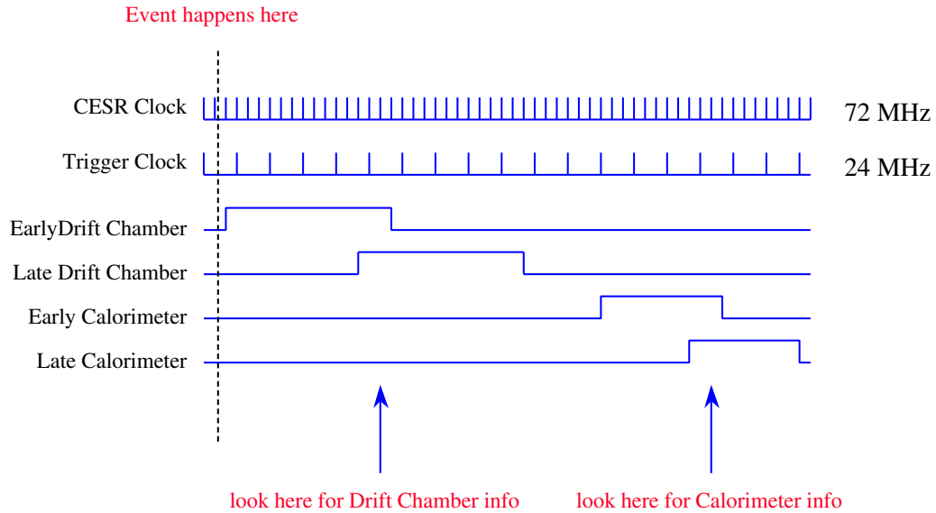
Figure 4.2: A diagram showing event timing in the CLEO III trigger.
