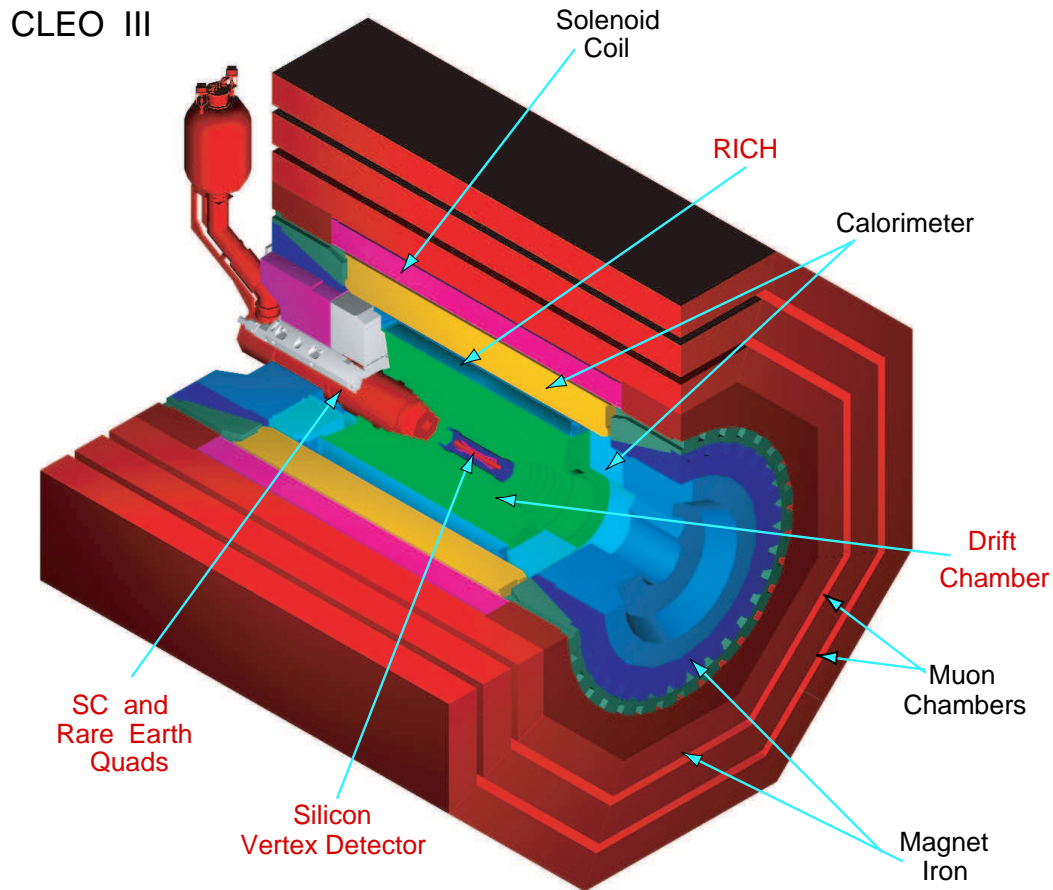
Figure 4.1: A view of the CLEO III detector.
