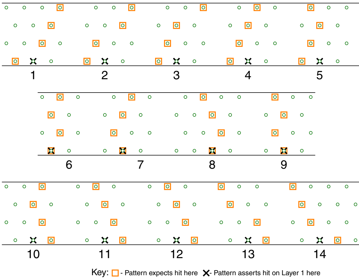
Figure B.1: The fourteen patterns for super layers 1 through 7.
