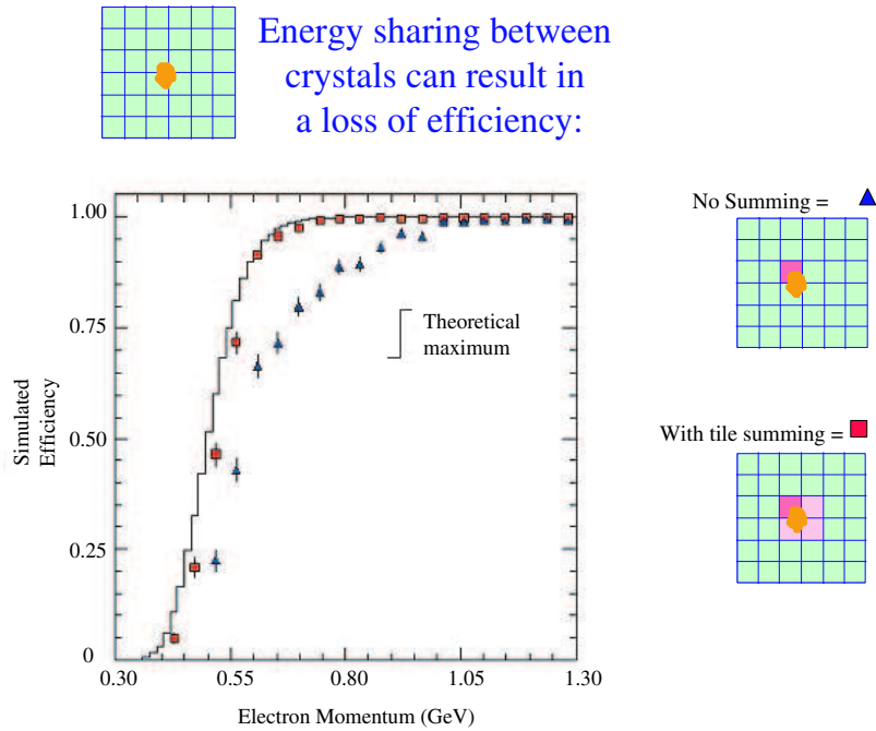
Figure 4.5: A turn-on curve with and without tile summing.
