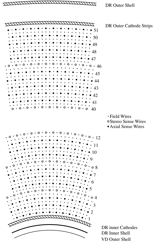
Figure 2.6: A diagram of the Main Drift Chamber.
