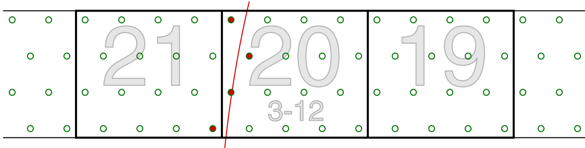
Figure 4.10: Here we have blocks 19 through 21 in superlayer 6 (see top center of Figure 4.12 to see where the blocks are in the Drift Chamber). The green circles are the wires that make up the blocks. These three blocks are fed information about their 48 wires by a single TQT card (in crate 3 slot 12). The red line is a track traversing the drift chambers with the red-filled circles being the wires that are hit.
