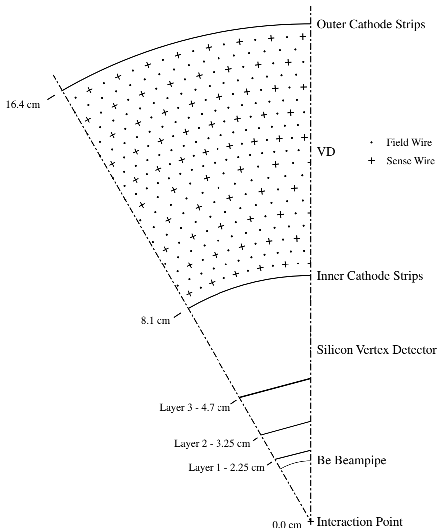
Figure 2.5: A diagram showing the relative positions of the Beam Pipe, Silicon Vertex Detector and the Vertex Detector.
