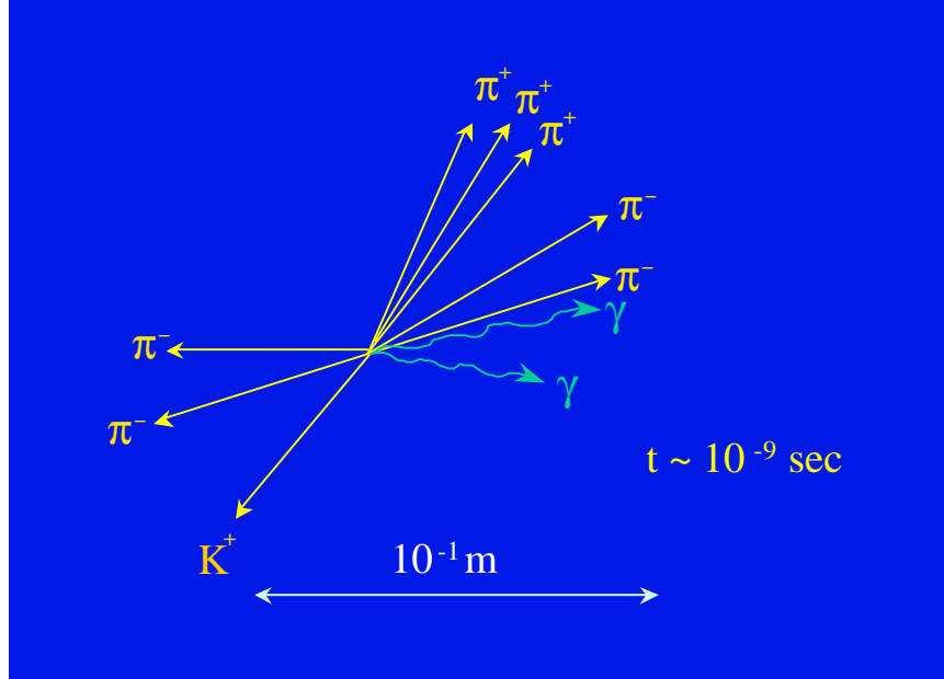
Figure 1.6: Particles have finally travelled far enough after about 10^{-9} seconds to be observed by the CLEO detector.
