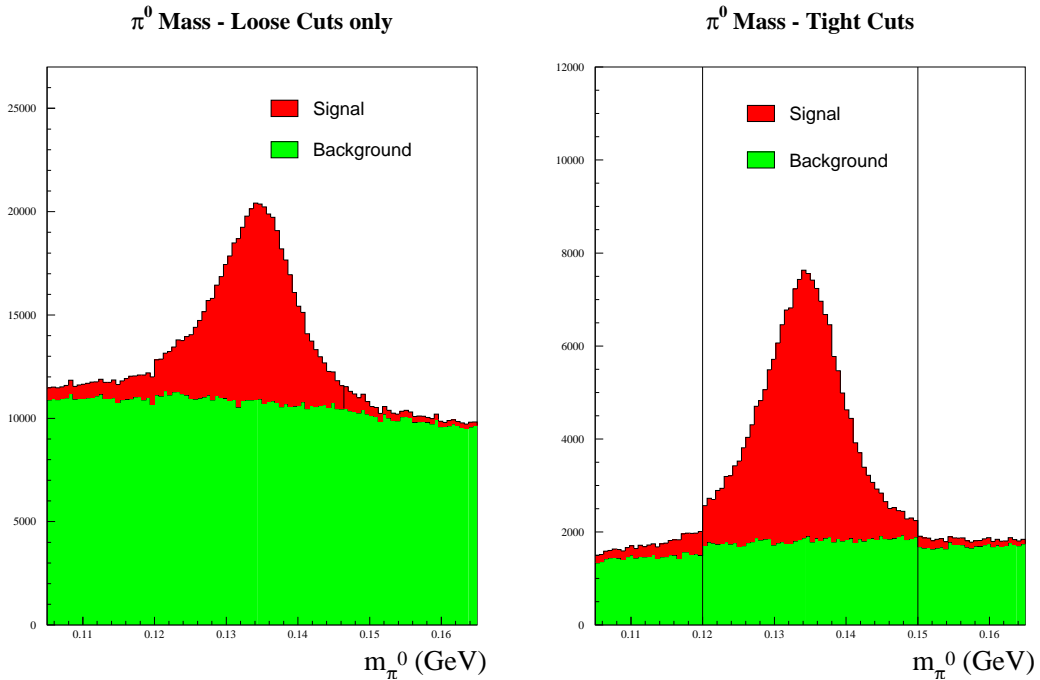
Figure 3.10: These two plots of reconstructed \pi^0 mass (the invariant mass of the two \gamma daughters) were generated from analyzing 100,000 MC events. The plot on the left shows real and fake \pi^0 s with only the CCFC cuts. The plot on the right is with all of our additional tighter cuts (except the mass cut). The vertical lines show the lower and upper mass cuts used in this analysis.
