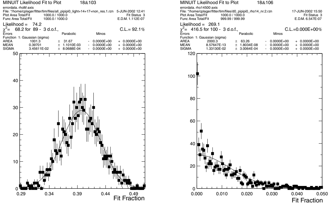
Figure 3.15: The fit of the \rho^- fit fraction distribution (left) and the fit of \rho_{1450}^0 fit fraction distribution (right), both from a set of 1000 trials where the matrix element parameters were varied according to the covariance matrix. For the \rho_{1450}^0 , the distribution is not well represented by a Gaussian. In this case, we quote a zero fit fraction with the error given by the Gaussian fit.
