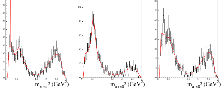
D^0 \rightarrow \pi^- \pi^+ \pi^0 Data - X projections D^0 \rightarrow \pi^- \pi^+ \pi^0 Data - Y projections D^0 \rightarrow \pi^- \pi^+ \pi^0 Data - Z projections
