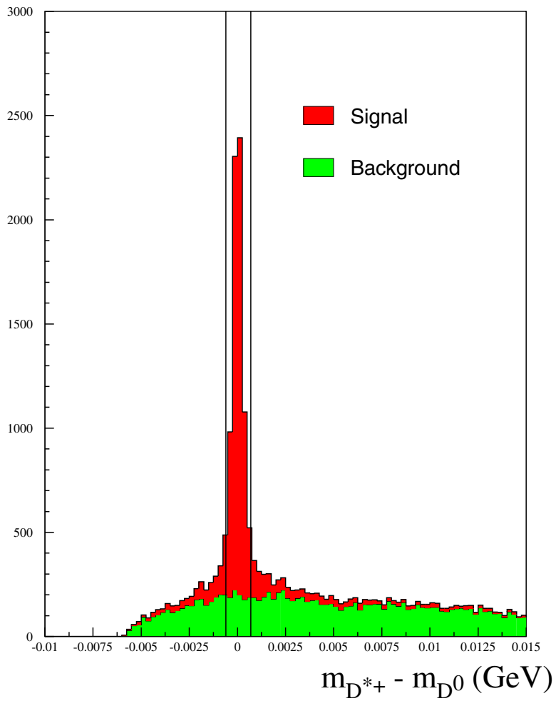
Figure 3.12: The analysis code was run on generic CLEO II.V MC (both b\bar{b} and continuum) and all cuts were used except the D^{*+} - D^0 mass difference cuts. The two vertical lines represent the lower and upper D^{*+} - D^0 mass difference cuts used in this analysis.
