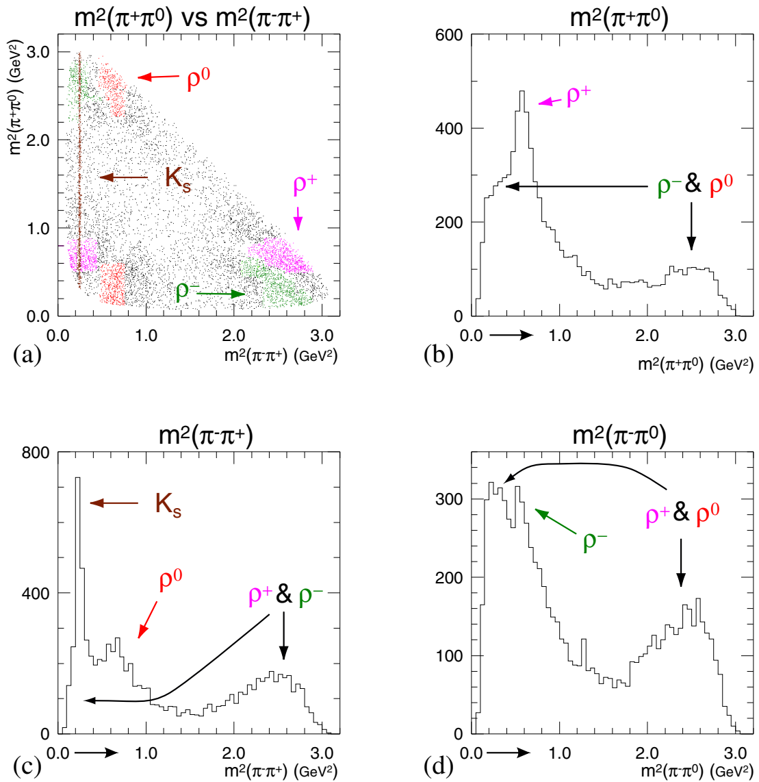
Figure 3.4: The D^0 \rightarrow \pi^- \pi^+ \pi^0 Dalitz plot (a) and the x (c), y (b), and z (d) projections. Note: All resonances are colored by hand for visualization.
