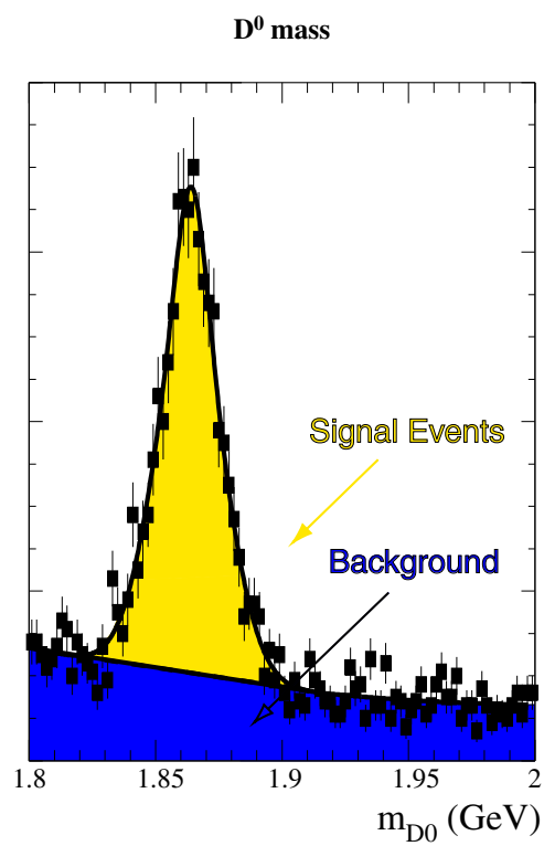
Figure 1.10: The distribution of D^0 mass in data using event selection criteria. The number of signal and background events can be determined by fitting this distribution to a background piece and a signal piece. See Section 3.7 for a more complete discussion about counting signal and background events.
