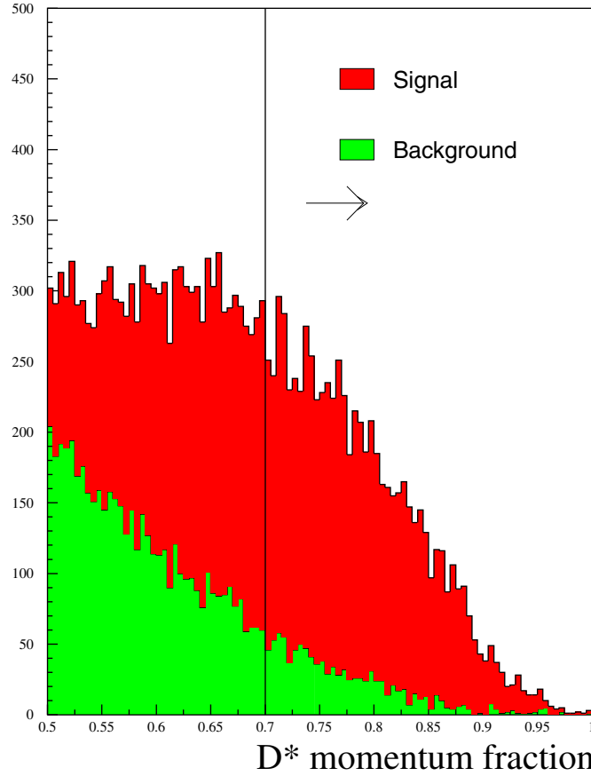
Figure 3.13: The analysis code was run on generic CLEO II.V MC (both b\bar{b} and continuum) and all cuts were used except the X_{D^*} cut. The vertical line represents the lower X_{D^*} cut used in this analysis..
