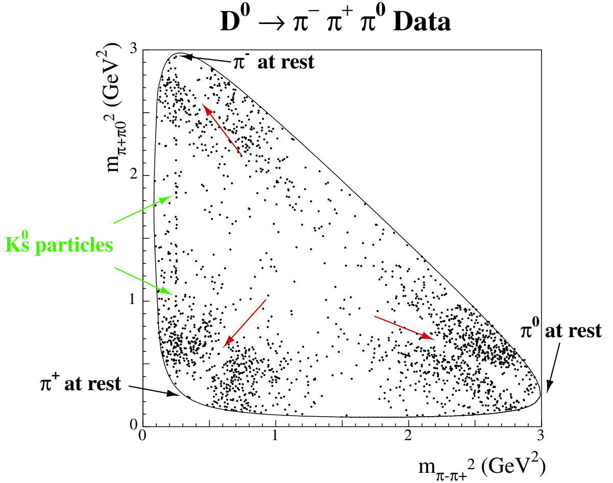
Figure 3.3: A plot of data from CLEO II.V of m_{\pi^+\pi^0}^2 versus m_{\pi^-\pi^+}^2 for reconstructed D^0 \rightarrow \pi^-\pi^+\pi^0 events. Note that each of the three corners is where one of the pions is at rest in the D^0 frame. The long thin vertical band on the left are K_S^0 . The colored arrows point to three regions on the Dalitz Plot where we can see destructive interference.
