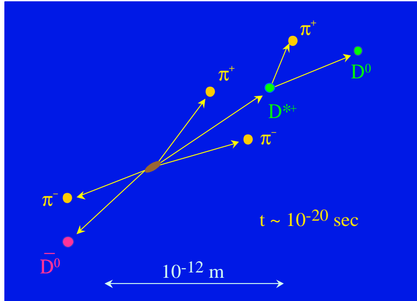
Figure 1.4: At t \approx 10^{-20} seconds, we have strong decays. In this case, the D^{*+} \rightarrow D^0 \pi^+ .
