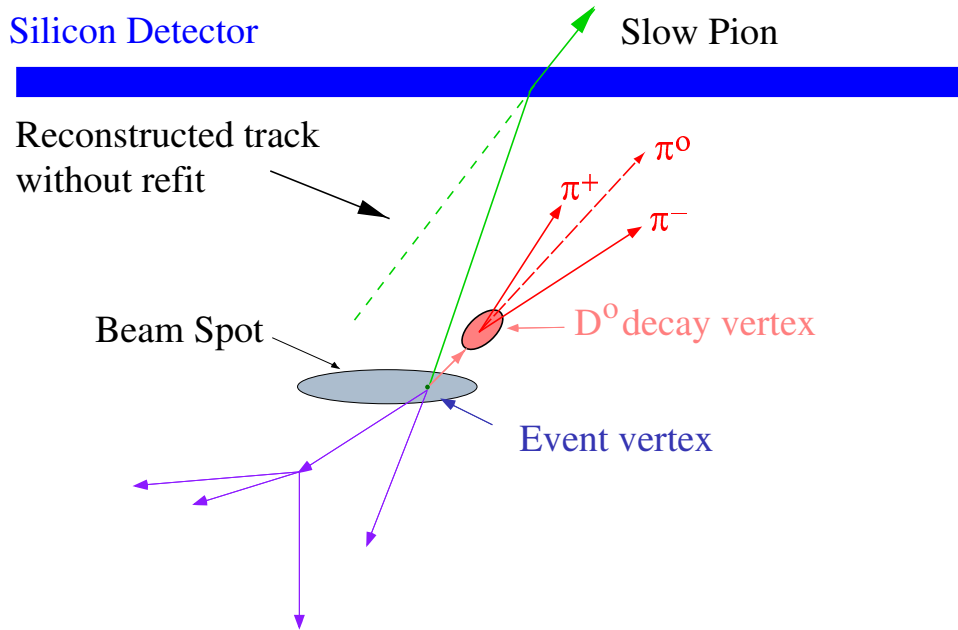
Figure 3.9: Using the D^0 and the beam spot we refit the slow pion. Note: We use the position information from the charged pions, not from the neutral \pi^0 , to calculate the vertex of the D^0 .
