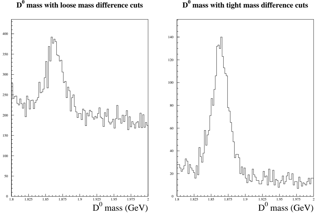
Figure 3.8: Shown are the D^0 mass distributions for loose mass difference cuts ( -10 \text{ MeV}/c^2 \leq \text{mass difference} \leq 15 \text{ MeV}/c^2 ) and tight mass difference cuts ( -0.6 \text{ MeV}/c^2 \leq \text{mass difference} \leq 0.7 \text{ MeV}/c^2 ) respectively.
