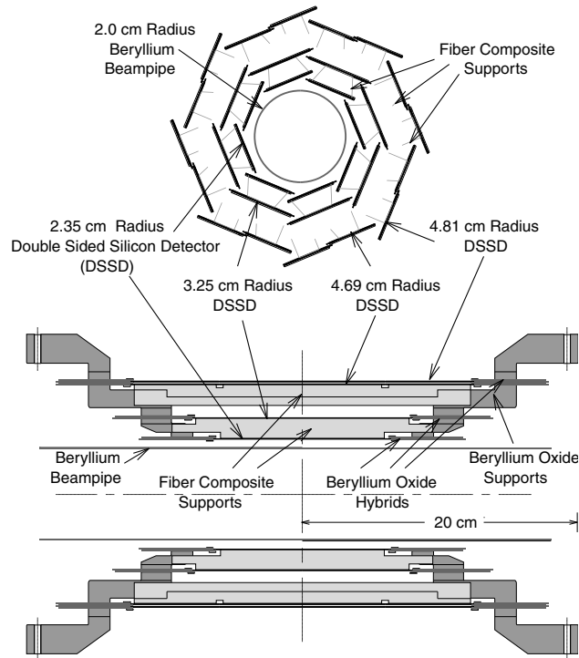
Figure 2.4: A view of the CLEO II.V Silicon Vertex Detector.
