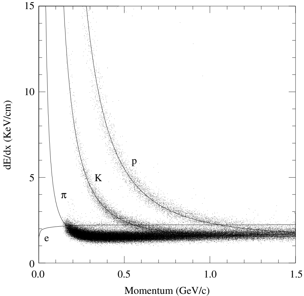
Figure 2.7: Energy loss per unit length of travel. The solid lines are averages for a given type of particle while the dots are data from real tracks. Notice that kaon-pion separation above 700 MeV is almost impossible.
