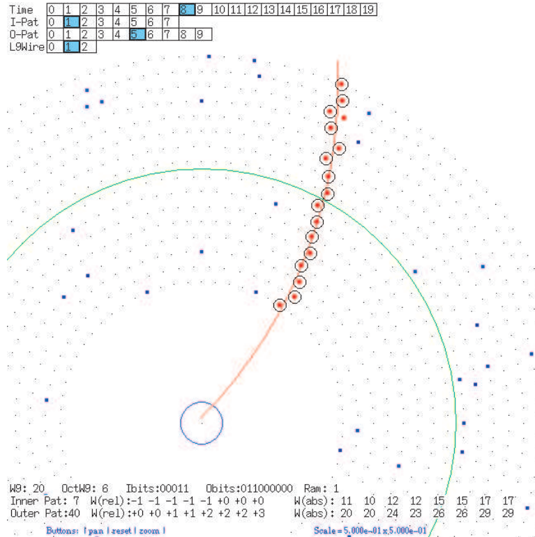
Figure 4.7: The AXTR looks at the inner eight and outer eight layers separately. In this case, since there is one hit per layer for the inner eight layers and at least one hit per layer in the outer eight layers, multiple patterns are satisfied.
