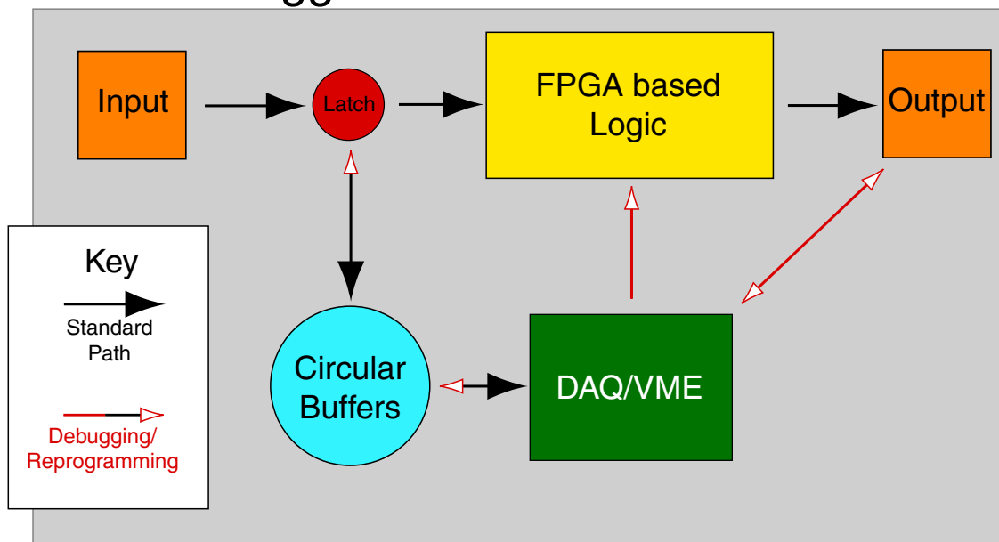
Figure 4.4: An overview of the general trigger board. The standard path is for the inputs to through a latch and go to both the trigger logic and the circular buffers. The outputs of the logic section then to the output connectors on the boards. For debugging purposes, we can fill the circular buffers from the VME interface, forcing the bits through the trigger logic and putting the output back into the VME interface. We can also use the VME interface to reprogram some of the logic FPGAs. Last but not least, we can also use VME to set various output patterns to test the output connector, the cables, and the input connectors of the next board.
