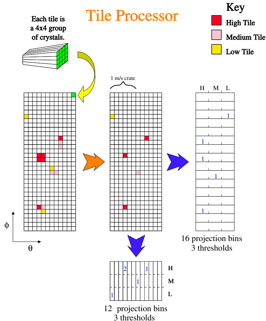
Figure 4.6: The Tile Processor takes care of both over-counting and making \phi and \theta projections.
