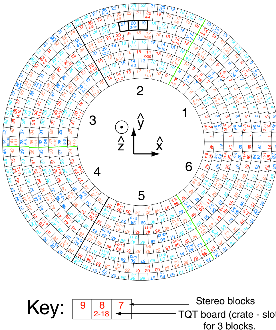
Figure 4.12: The map of stereo blocks (U super layers in red; V superlayers in blue). The beam pipe is coming out of the middle of the circle (along \hat{z} ). Each three blocks gets its signal from a TQT board. Superlayer 6 blocks 19 through 21 are highlighted since they are the example in Figure 4.10. The three thick black lines (at 3 o'clock, 7 o'clock and 11 o'clock) are boundaries of the three-fold symmetry as well as STTR board boundaries. The thick green lines are STTR board boundaries. The numbers "1" through "6" on the inside refer to the regions covered by the stereo boards (6 U boards and 6 V boards).
