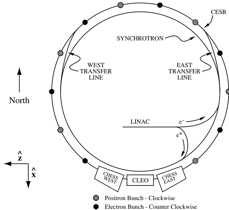
Figure 2.1: A layout of CESR. Note that “up” is North, \hat{x} is South and \hat{z} is West.
