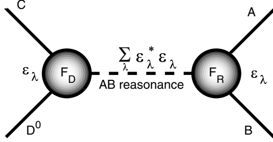
Figure 3.1: A representation of D^0 \rightarrow ABC through an AB resonance. Since the initial and final states have no angular momentum, the intermediate spin states are summed over.
