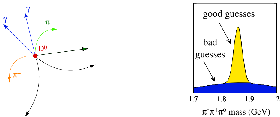
Figure 1.8: A D^0 mass distribution assuming every event has the decay chain we are looking and that other charged and neutral particles are also present.
