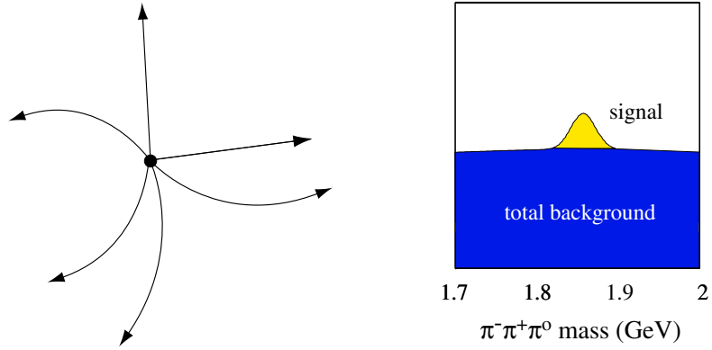
Figure 1.9: A D^0 mass distribution assuming some events have the decay chain we are looking for, but most do not.
