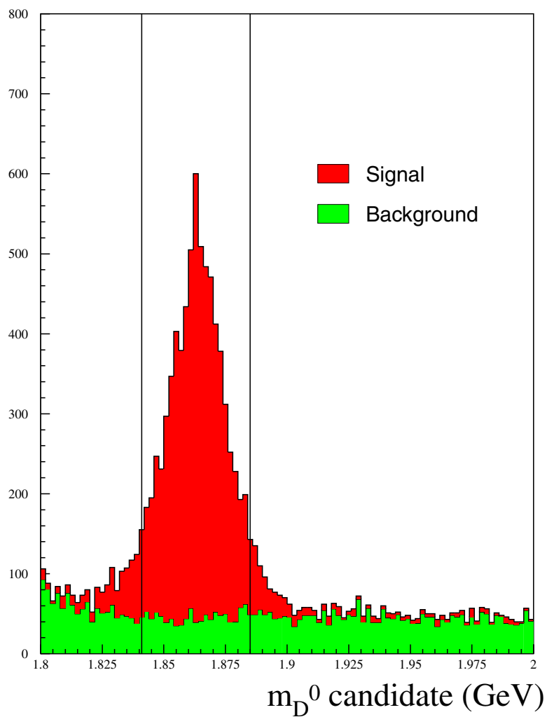
Figure 3.11: The analysis code was run on generic CLEO II.V MC (both b\bar{b} and continuum) and all cuts were used except the D^0 mass cuts. The two vertical lines represent the lower and upper D^0 mass cuts used in this analysis..
