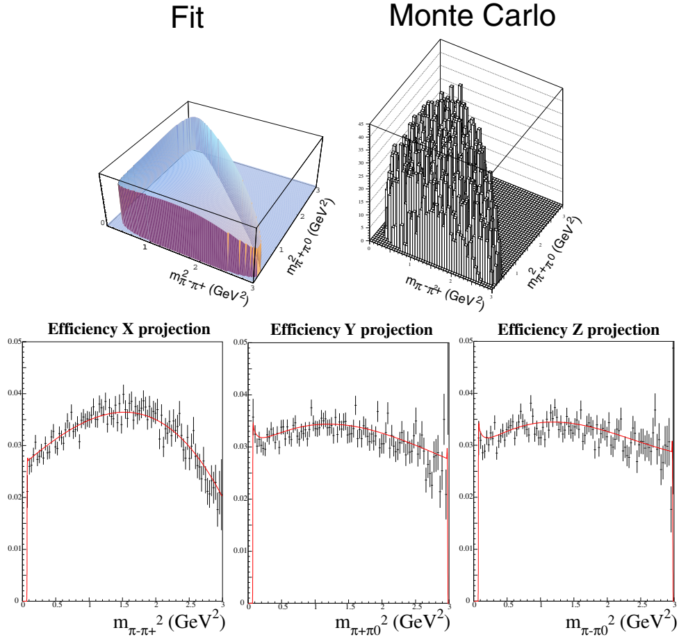
Figure 3.16: The best efficiency function and the Monte Carlo to which it was fit. For the projections, the red line is the fit and the black histogram is the MC. Note: The efficiency for each bin is normalized by the height of that bin.
