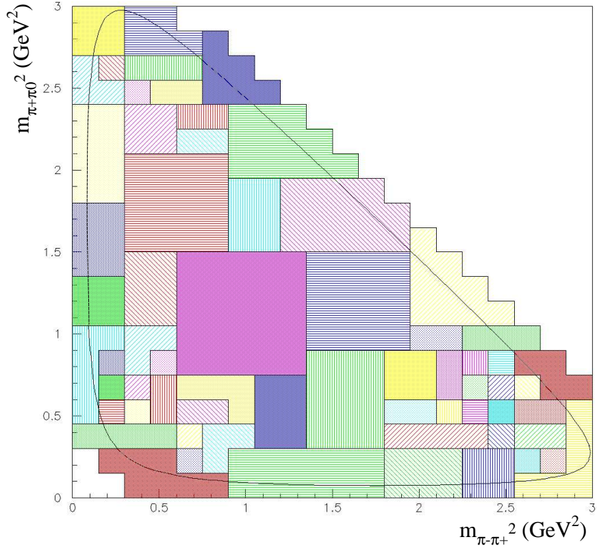
Figure 3.14: The binning that we will use to calculate \chi^2 goodness of fit. We started with bins of 150 \text{ MeV} per side and combined bins until each had a minimum of 20 data events.
