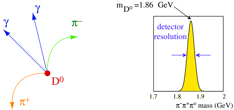
Figure 1.7: A D^0 mass distribution assuming there is nothing in the events except the particles we are looking for. The width of the distribution is a measure of detector resolution since the intrinsic width of the D^0 is so small.
