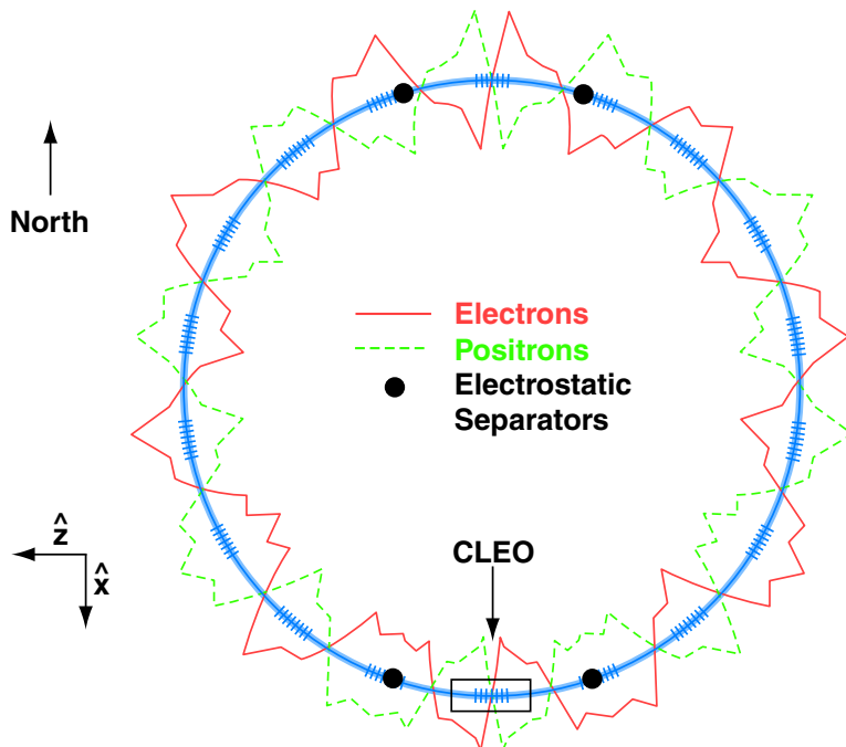
Figure 2.2: A diagram of CESR pretzel orbit. The extent to which the orbit deviates from circular is greatly exaggerated for illustration purposes.
