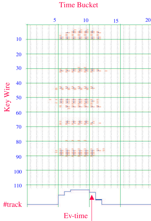
Figure 4.9: The AXPR calculates event time by watching the number of the 112 key wires that are hit.
