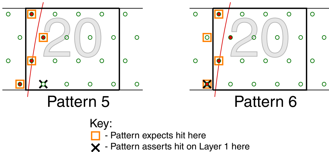
Figure 4.11: Continuing with the example in Figure 4.10, we have four wires hit in/near block 20. In this case, two different patterns are satisfied (pattern 5 has four out of four wires hit while pattern 6 has only three out of four wires hit). In this case there is a problem because the two different patterns would set two different blocks as being hit, violating the second constraint.
