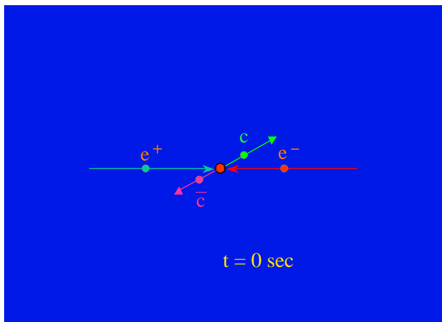
Figure 1.2: e^+e^- \rightarrow c\bar{c} .
