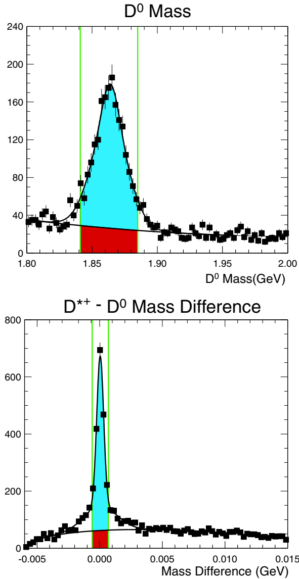
Figure 3.19: The distributions for the D^0 mass and the D^{*+} - D^0 mass difference (centered at the PDG value). These two plots were made with all cuts except the D^0 mass cuts for the upper and mass difference cuts in the lower. The green lines are the upper and lower cuts. In both plots, the area of the upper blue region is our estimation of signal events while the red area represents background events.
